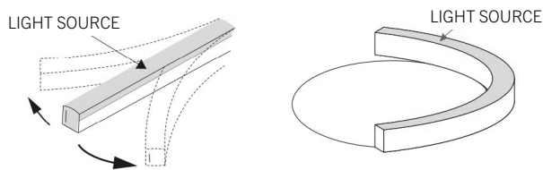
HORIZONTAL BEND
