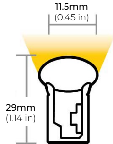
DOME LENS
