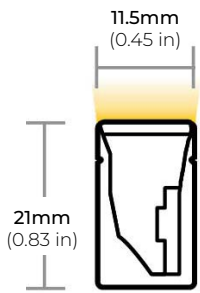
FLAT LENS
